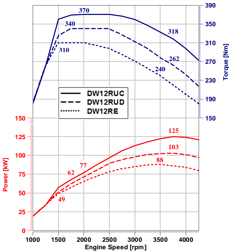
Performances curves
